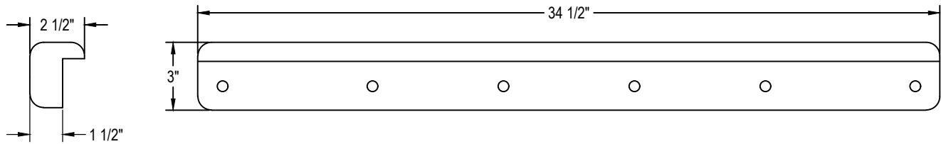
SIDE
